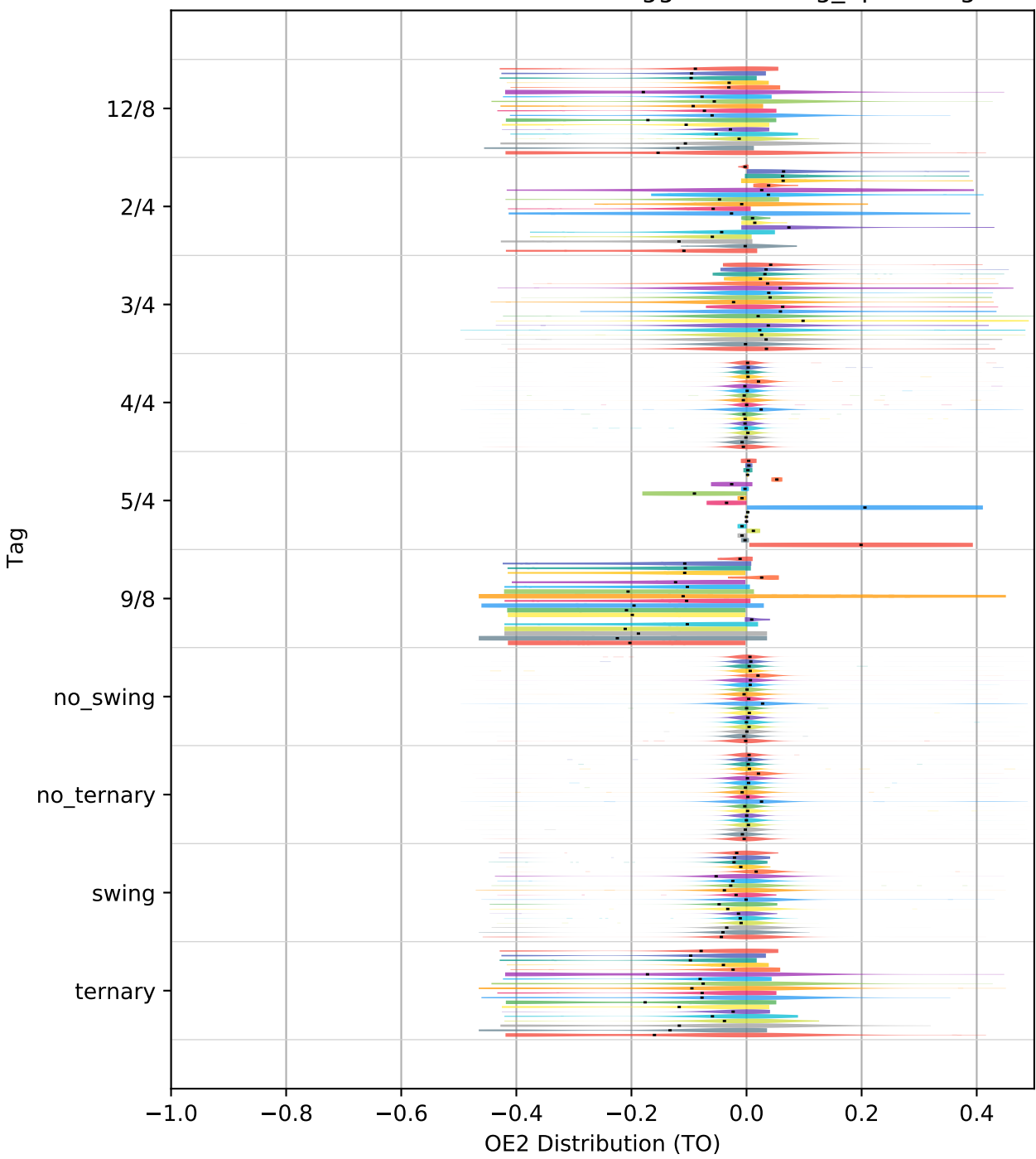
OE2 Distributions for Tracks Tagged with 'tag_open' Tags
