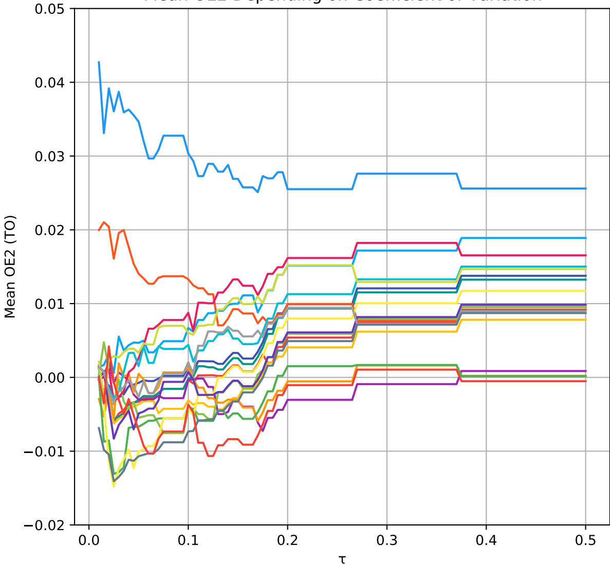
Mean OE2 Depending on Coefficient of Variation
