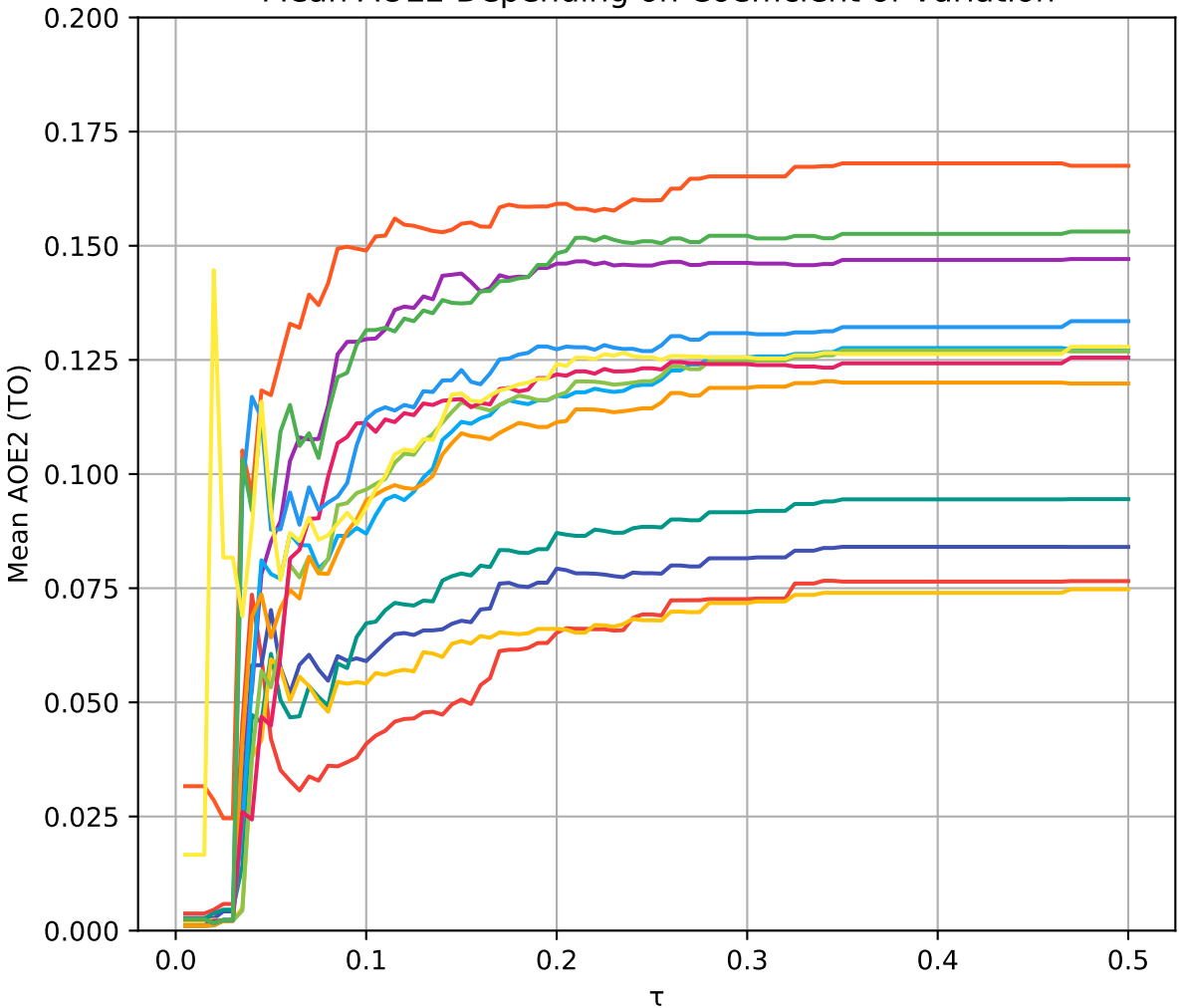
Mean AOE2 Depending on Coefficient of Variation
